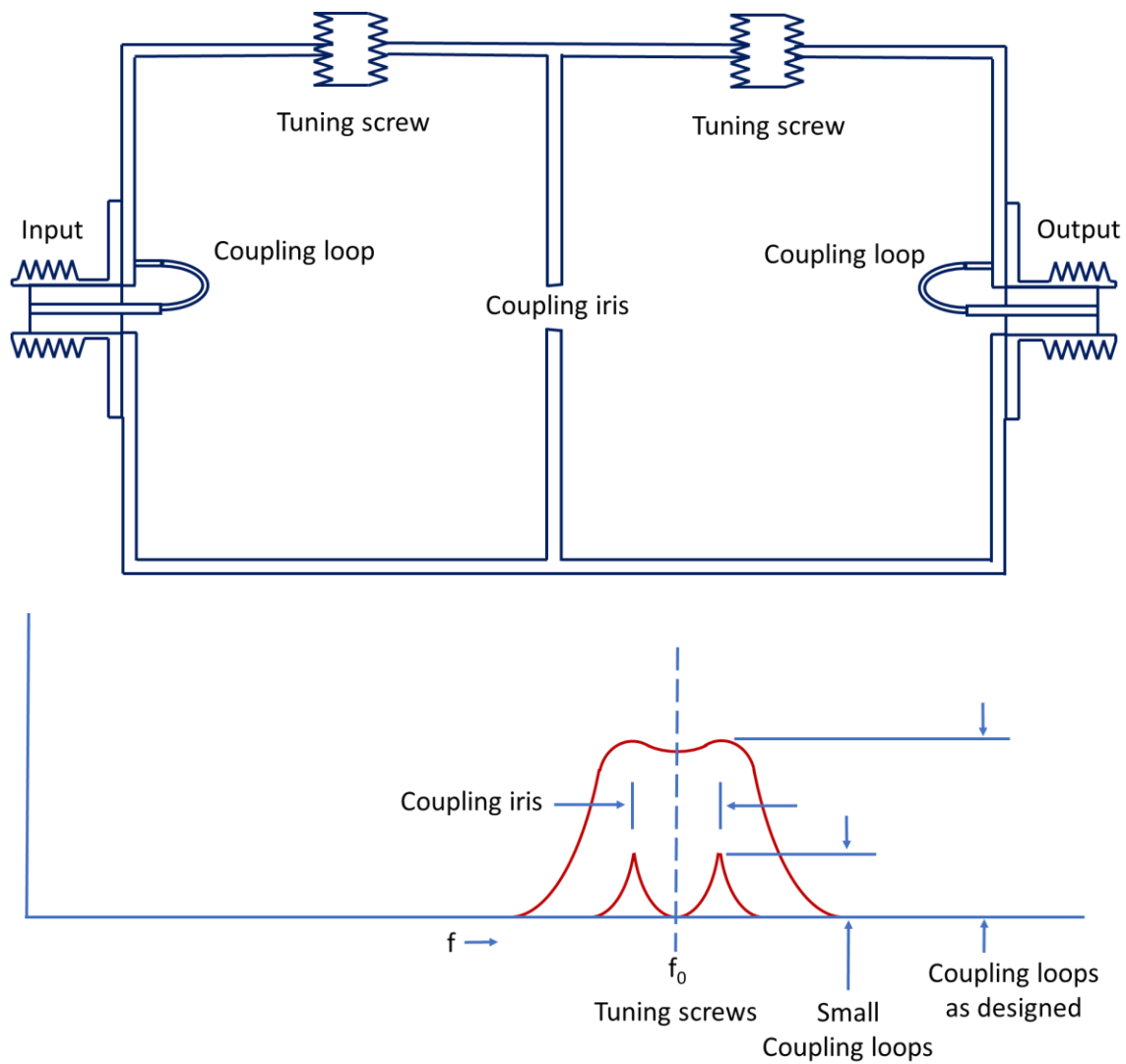
Figure 12: Two-section microwave bandpass filter cross-section and frequency response
