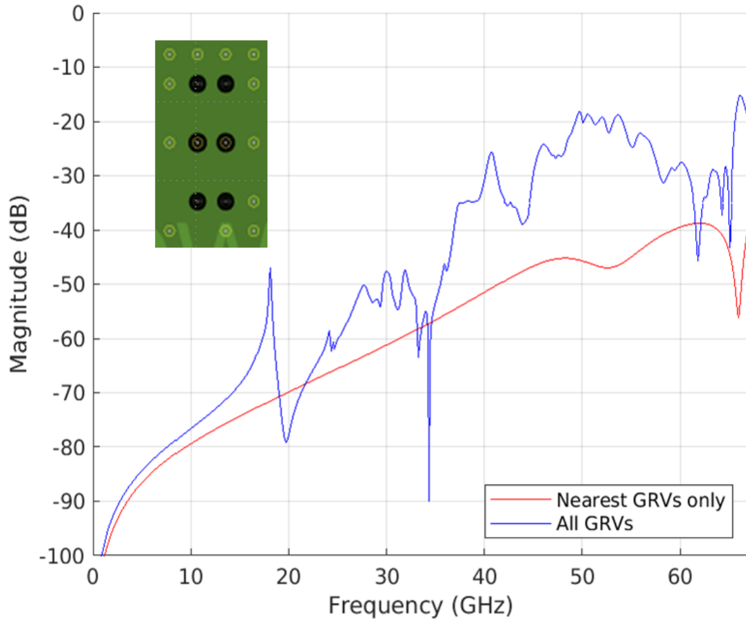
Figure 8: Site 8 near end differential crosstalk vs. GRV Population
