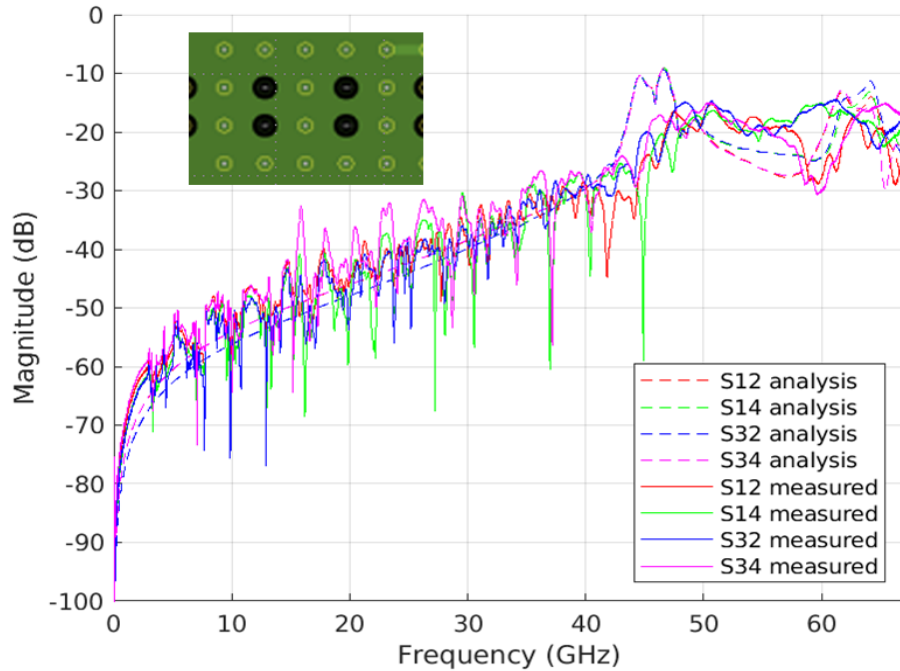
Figure 11: Site 3 measured and modeled single-ended response
