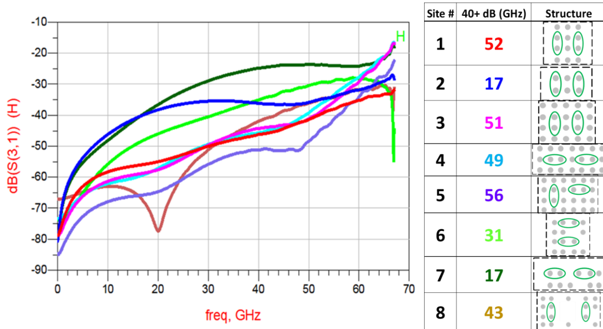
Figure 4: Differential Crosstalk Measurements, by test site
