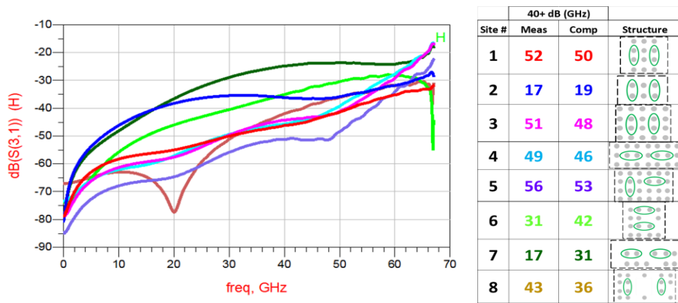
Figure 10: Gated measurement results (left) adding comparison of computational 40 dB crosstalk versus DSV/GRV structure (right).
