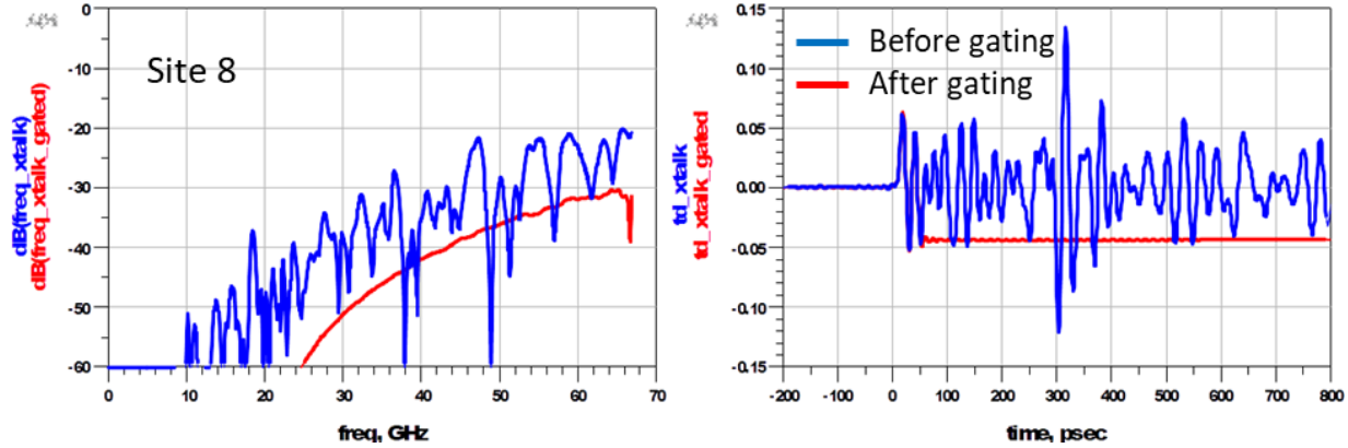
Figure 6: Measured Results, before and after gating
