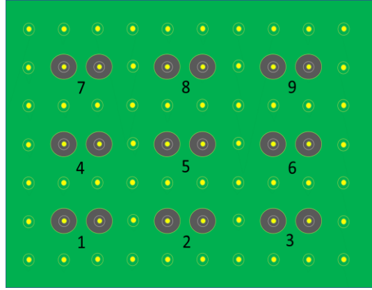
Figure 13: DSV locations for adjacent site crosstalk study
