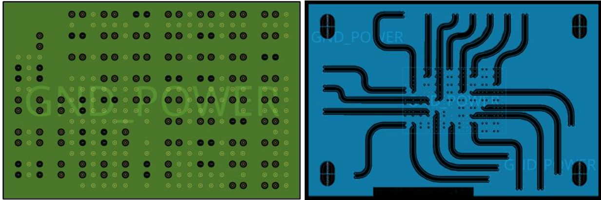
Figure 1: GRV Testboard Layout
