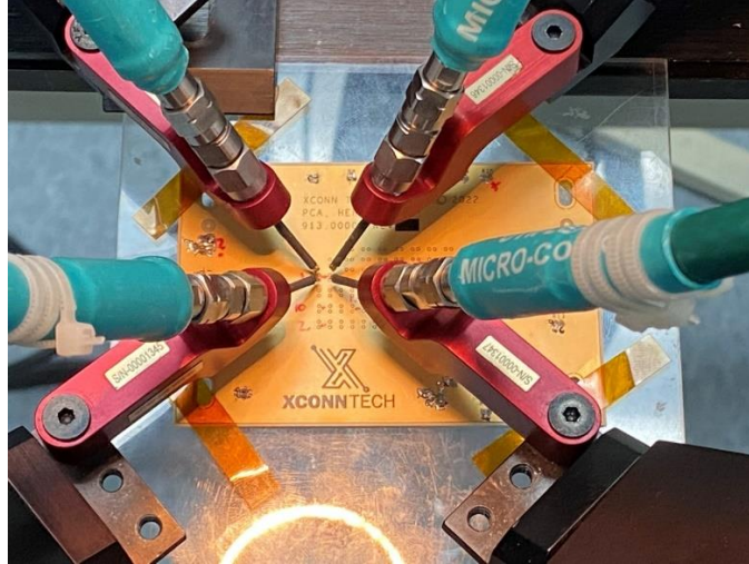
Figure 5: Measurement probes, applied to Testboard
