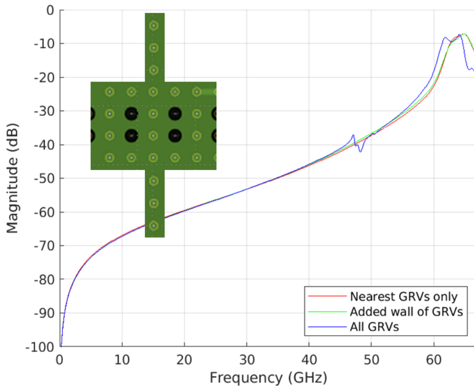
Figure 7: Site 3 near end crosstalk vs. GRV population
