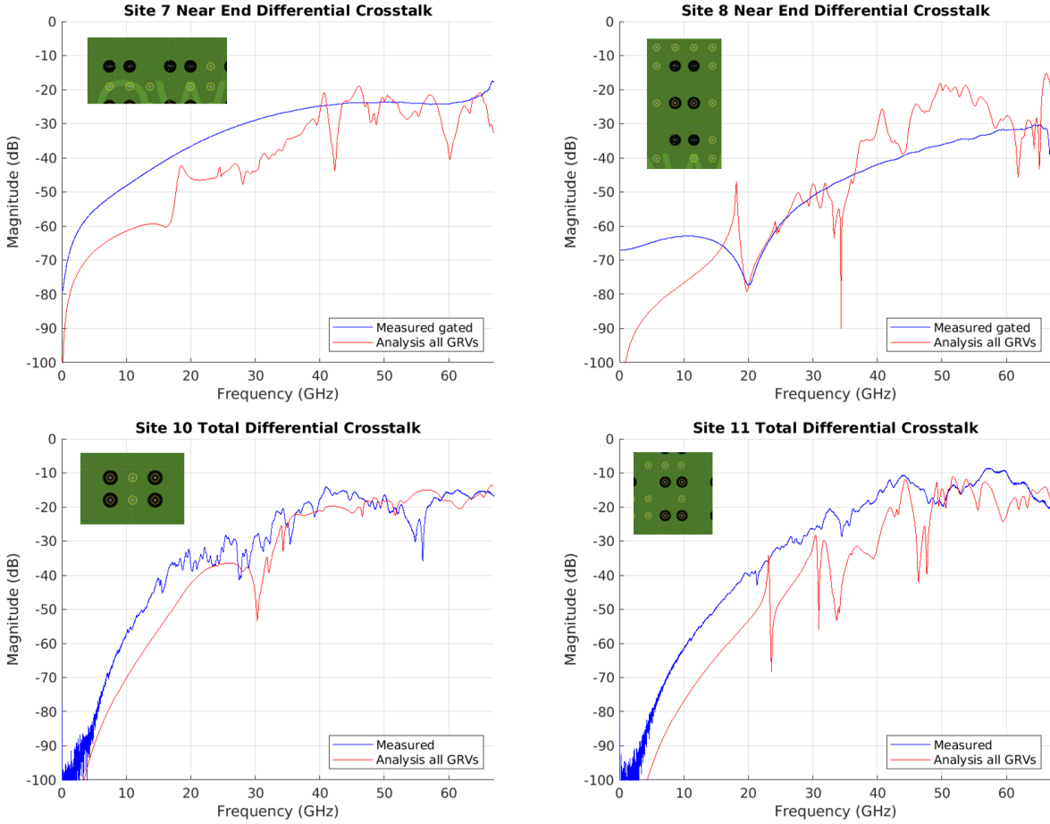
Figure 9: Gated measurement results compared to model with all GRVs
